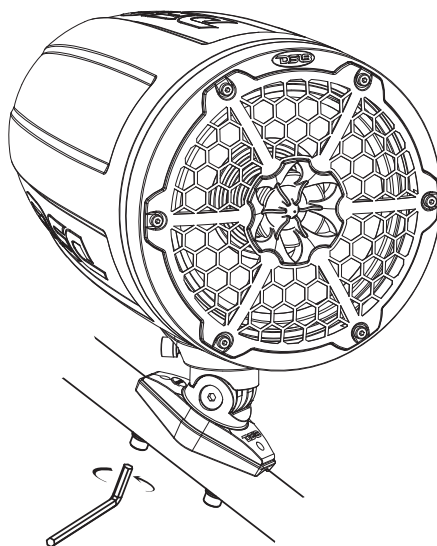
TUBE MOUNTING
