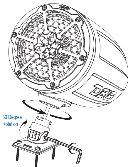
FLAT MOUNTING
