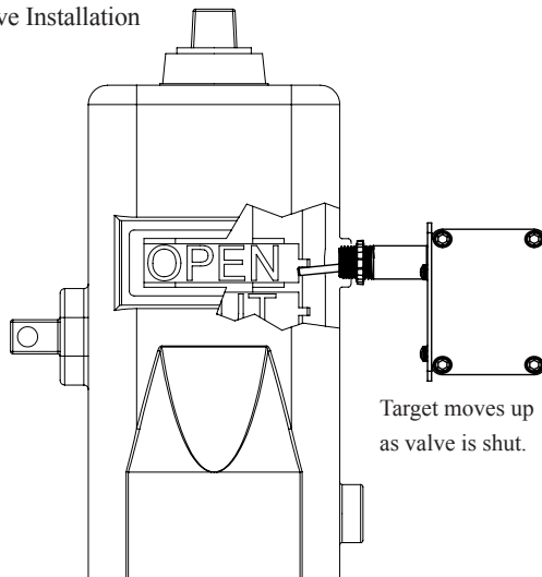
Typical Valve Installation Fig 4
