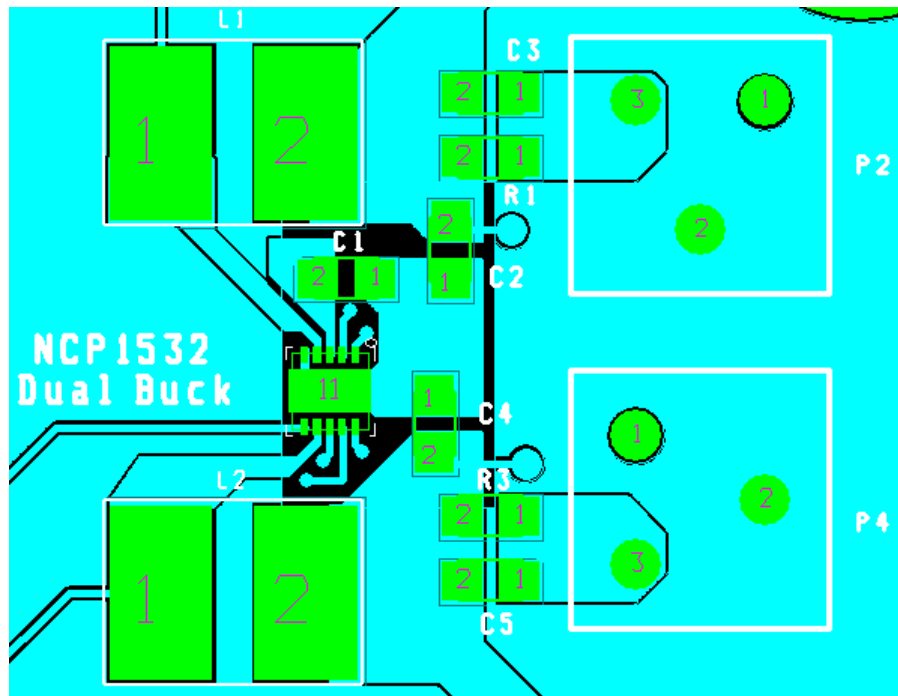
Figure 8. Part Layout
