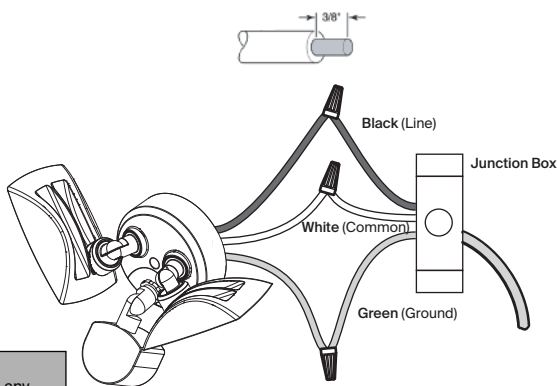
Non-Dimming Wiring Diagram
