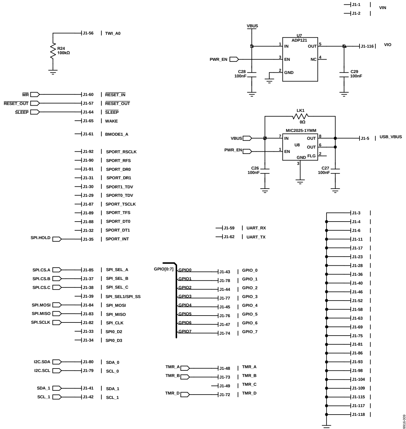
Figure 9. SDP-S—Connector
