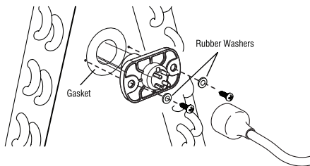
Fig. 3. Insert lamp into delta plate hole and secure with screws and washers. Connect remote lamp power cord.
