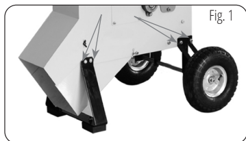
Attaching the leg
