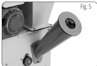
Funnel installation
