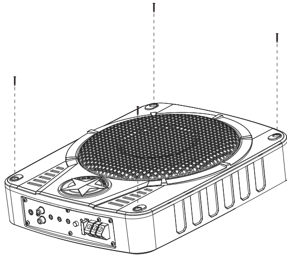
Mounting Amplifier
