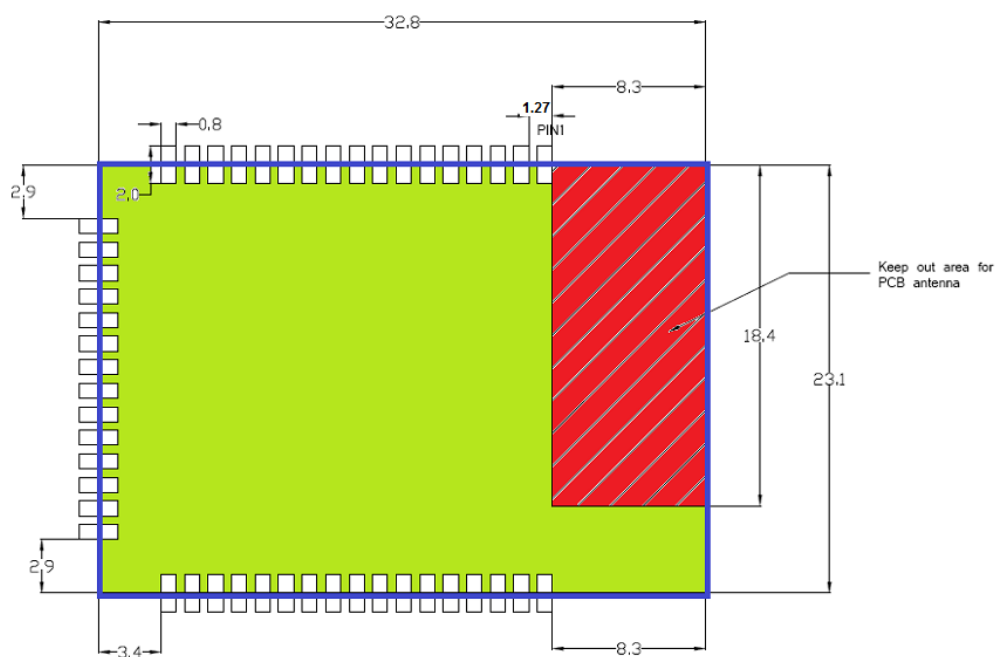
Figure 4. MYK2011_100 PCB Symbol Size
