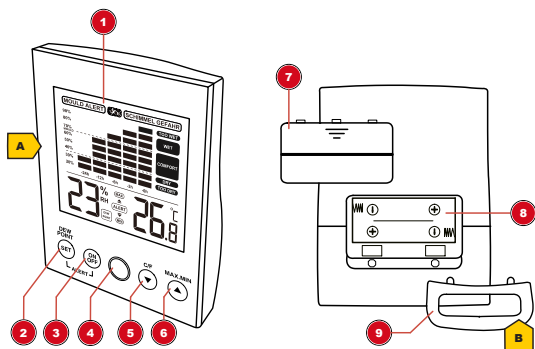
Illustration 1: Hygrometer parts overview
