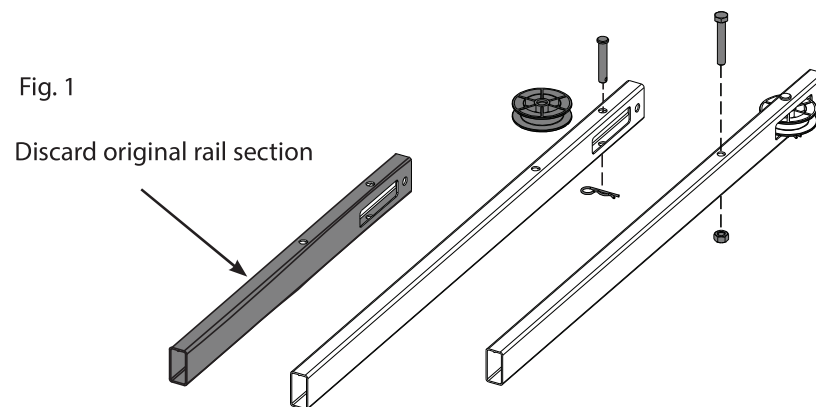
Extended rail section step 1a & 1b from assembly poster
