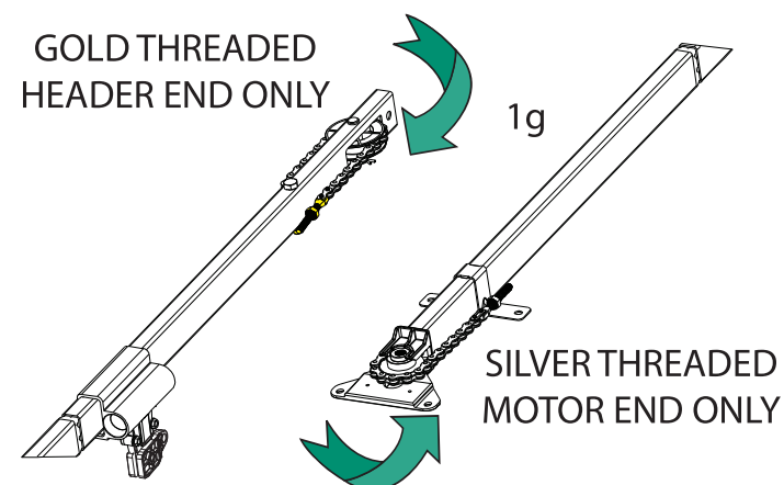
Fig. 4 Continue at step 1g from assembly poster
