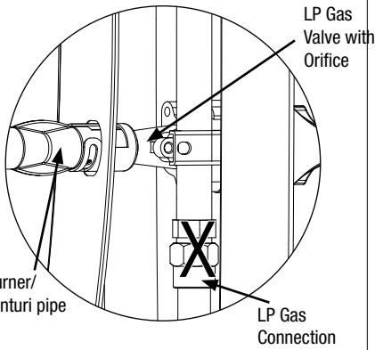
Figure 1: Main Burners
