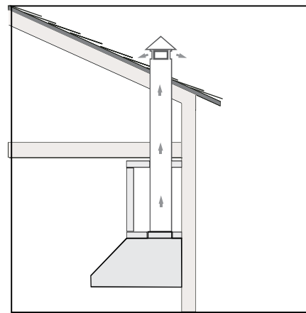
ROOF EXHAUST
