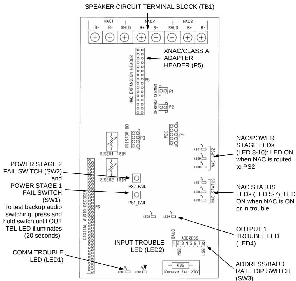
Figure 1. Flex Amplifier without CSNAC Compatibility
