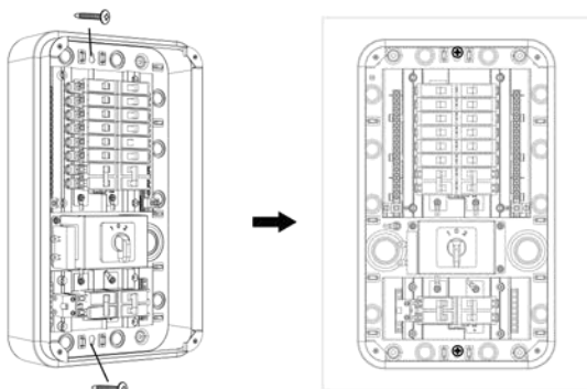
Figure 2.3.2 Drill & Mount
