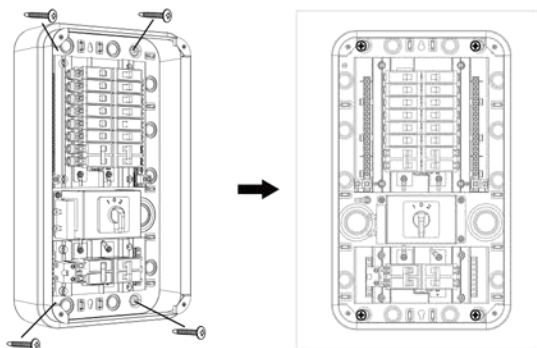
Figure 2.3.1 Drill & Mount
