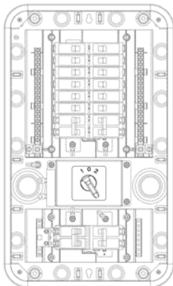
Figure 4.2 Machine power
