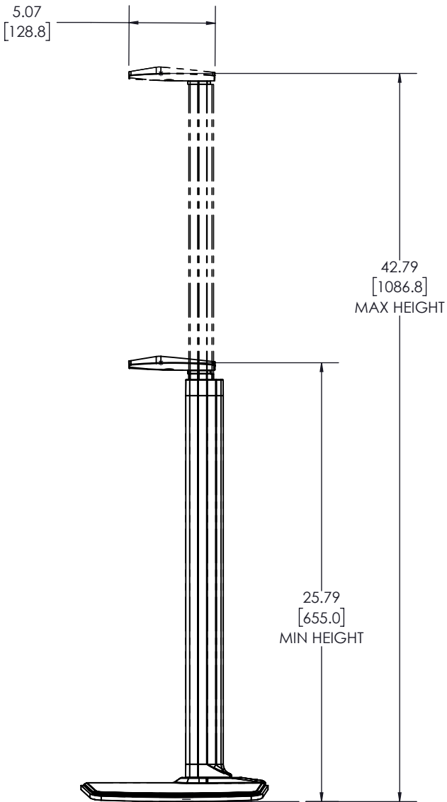
SIDE VIEW
