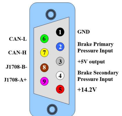
Bus side DB9 male connector
