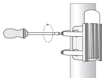
Pole Mount
