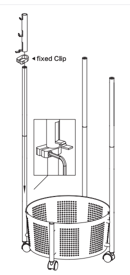
3.Install fixed clip and put the rotary tube in, one rotary tube must have one fixed clip to avoid it run up and down.
