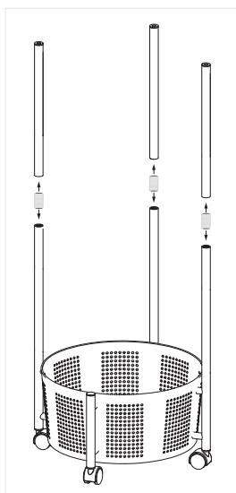
2.Install the upper pipe section and lock the joint connection through the screw thread
