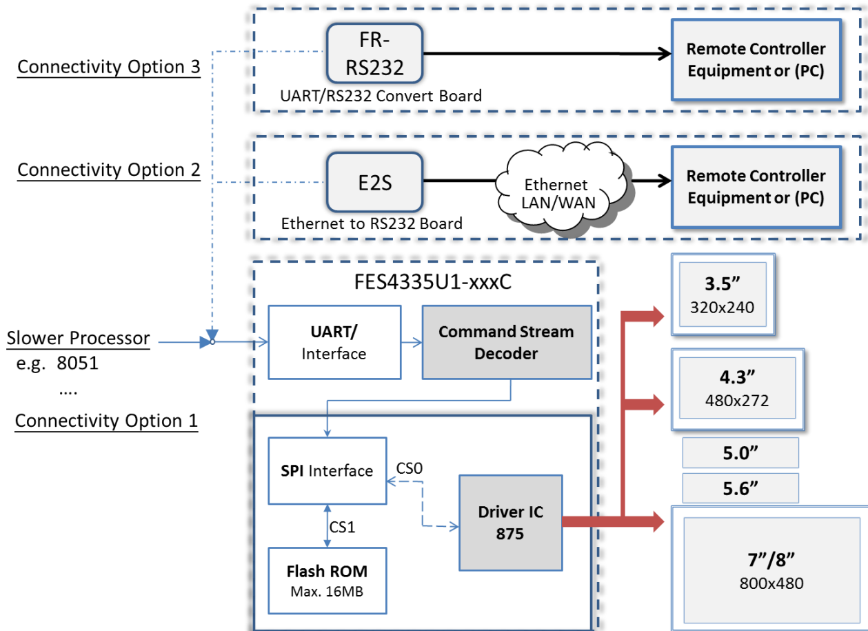
Figure 3-a : The Block Diagram of FES4335U1-xxC
