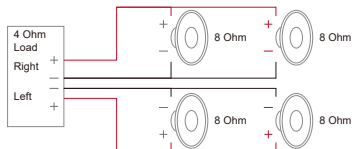
Parallel Speaker wire Diagram
