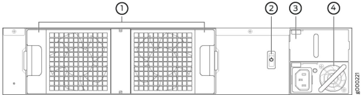
Figure 2: Rear Panel of the JA2500 Appliance
