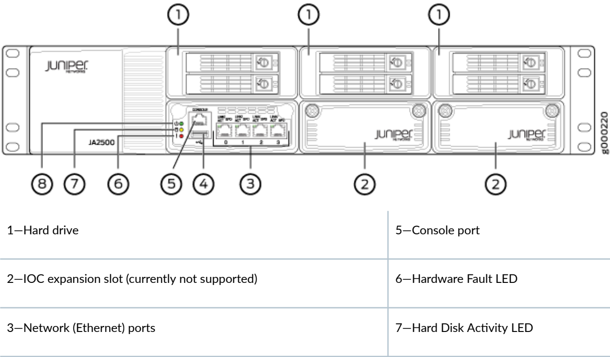
Figure 1: Front Panel of the JA2500 Appliance
