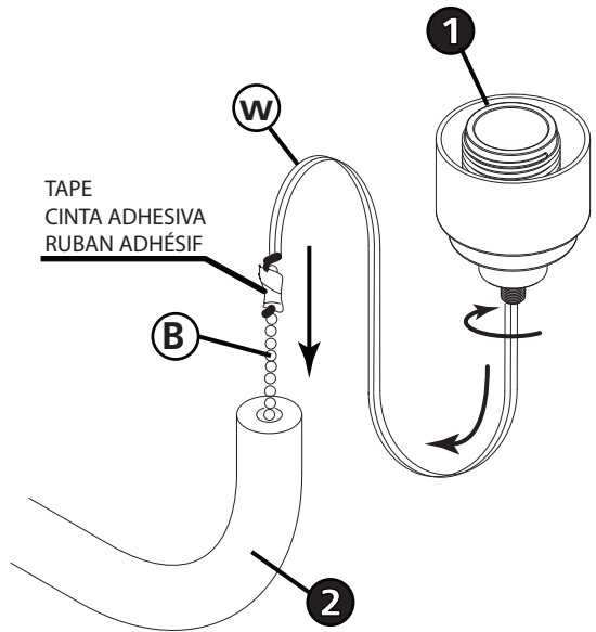
DRAWING 1 - ASSEMBLY
