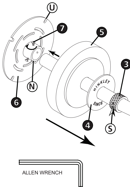
DRAWING 2 - ASSEMBLY
