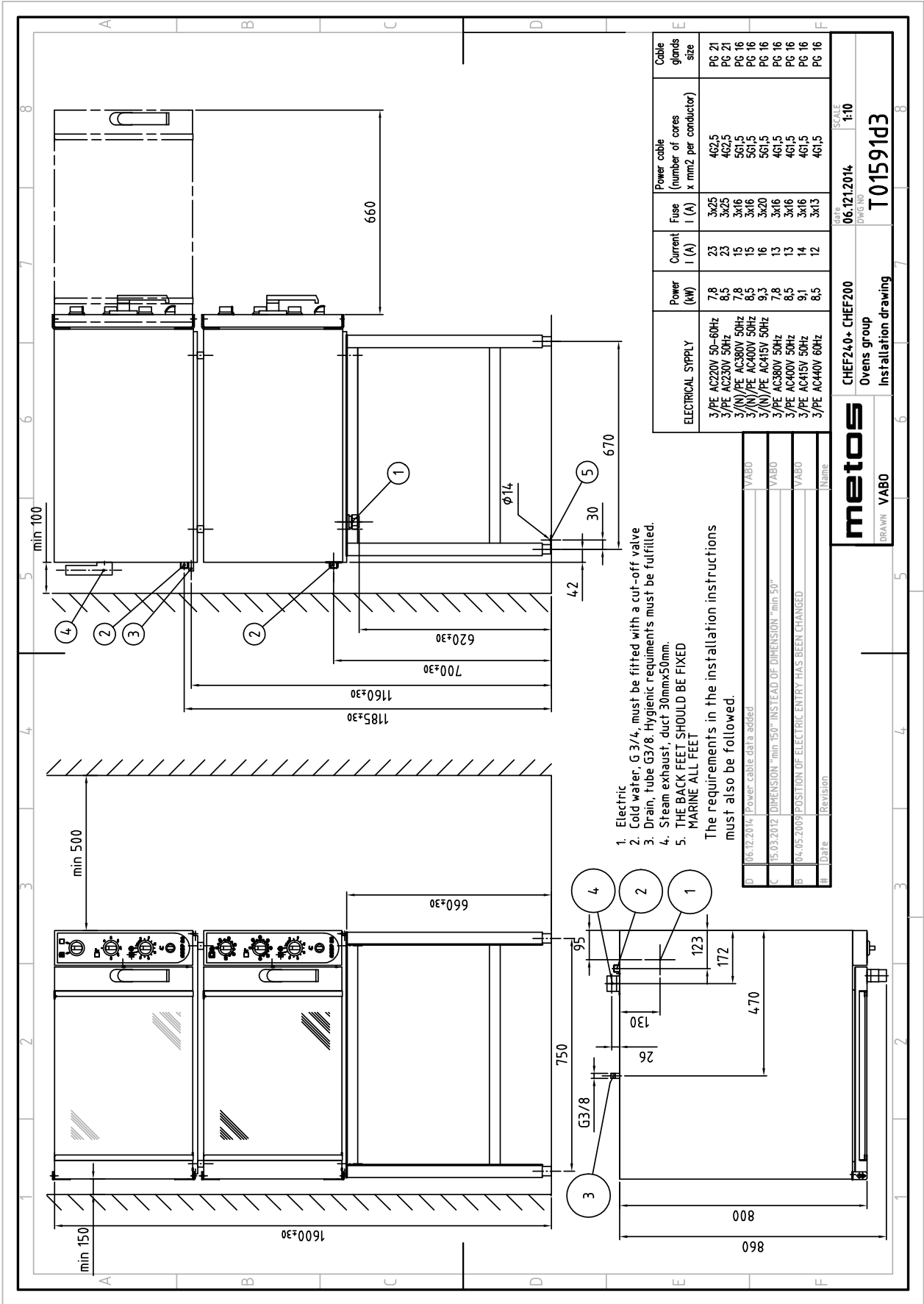
Installation drawing T01591D3
