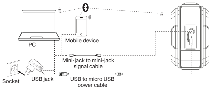
Fig. 2. Connection diagram
