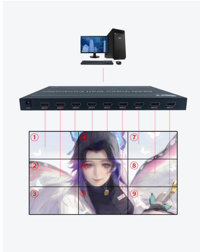
3x3 mode front panel wiring diagram (5760x3240@60Hz)
