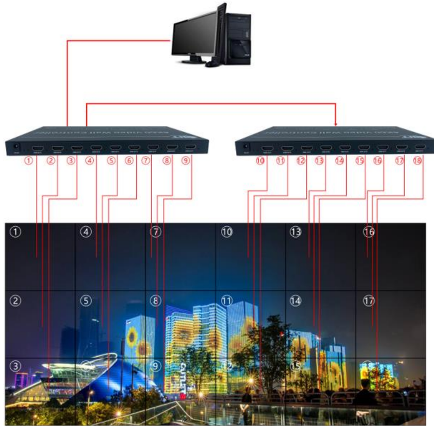
3x6 mode front panel wiring diagram (5760x6480@60Hz)
