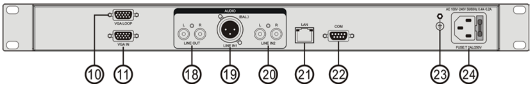
HCS-8316VGA-H 后面板
