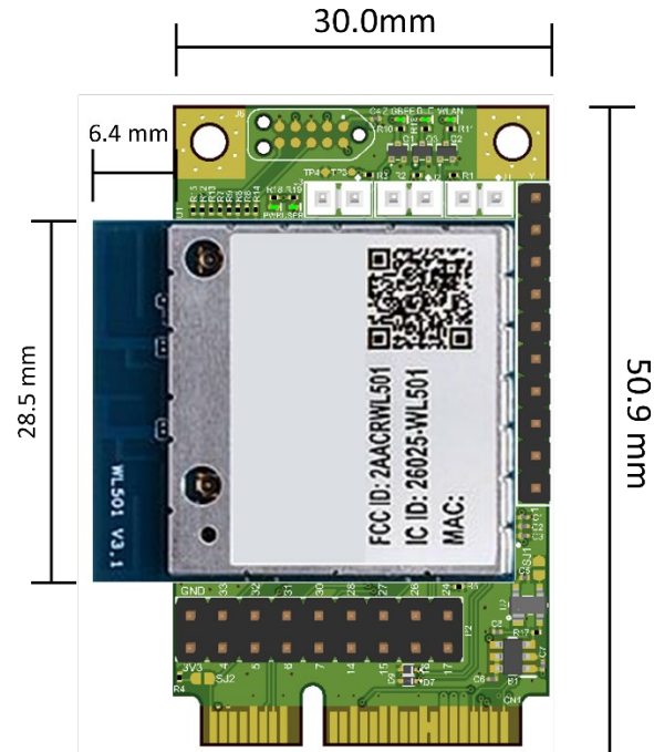
Figure 2: QCA4020 miniPCle Physical Dimension.
