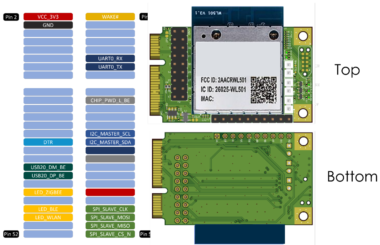
Figure 3: QCA4020 miniPCle Pin out.
