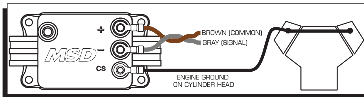
Figure 1 Coil Wiring.
