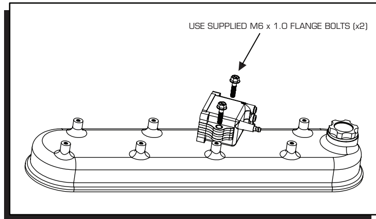
Figure 2 LS Valve Cover Mounting.
