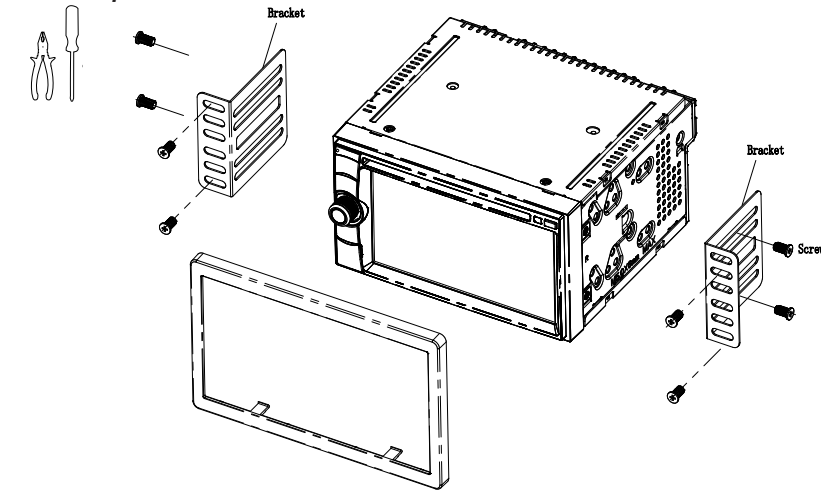
Typical front load ISO-DIN method
