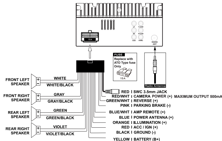
Typical front load ISO-DIN method
