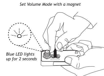
Set Volume Mode with a magnet
