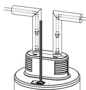
Typical horizontal piping arrangement
