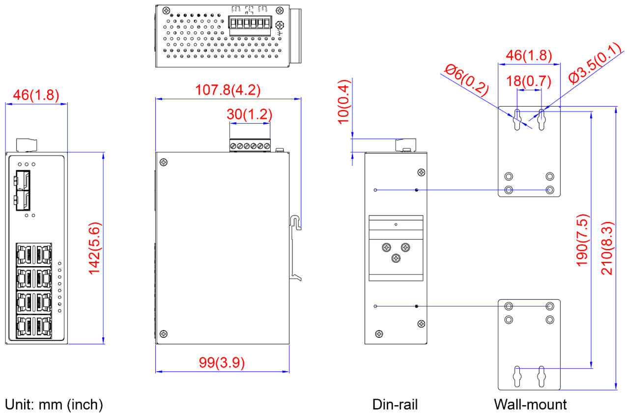
Figure 2.1: Physical Dimensions
