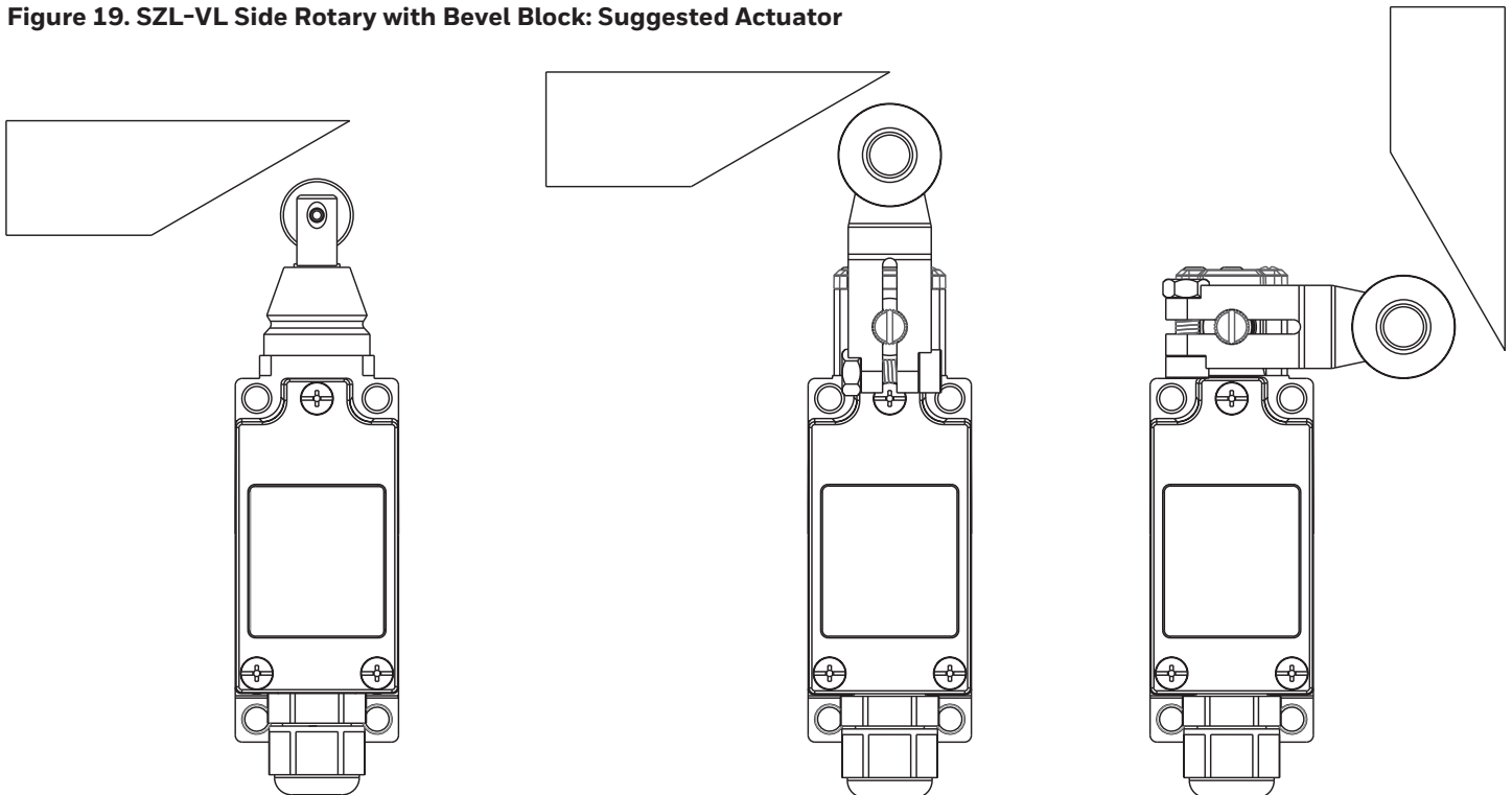
Figure 19. SZL-VL Side Rotary with Bevel Block: Suggested Actuator
