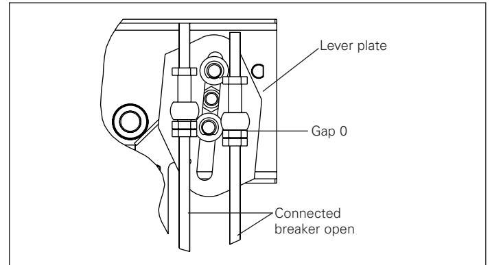
Figure 14. Driven "And" lever position with interconnected breakers open
