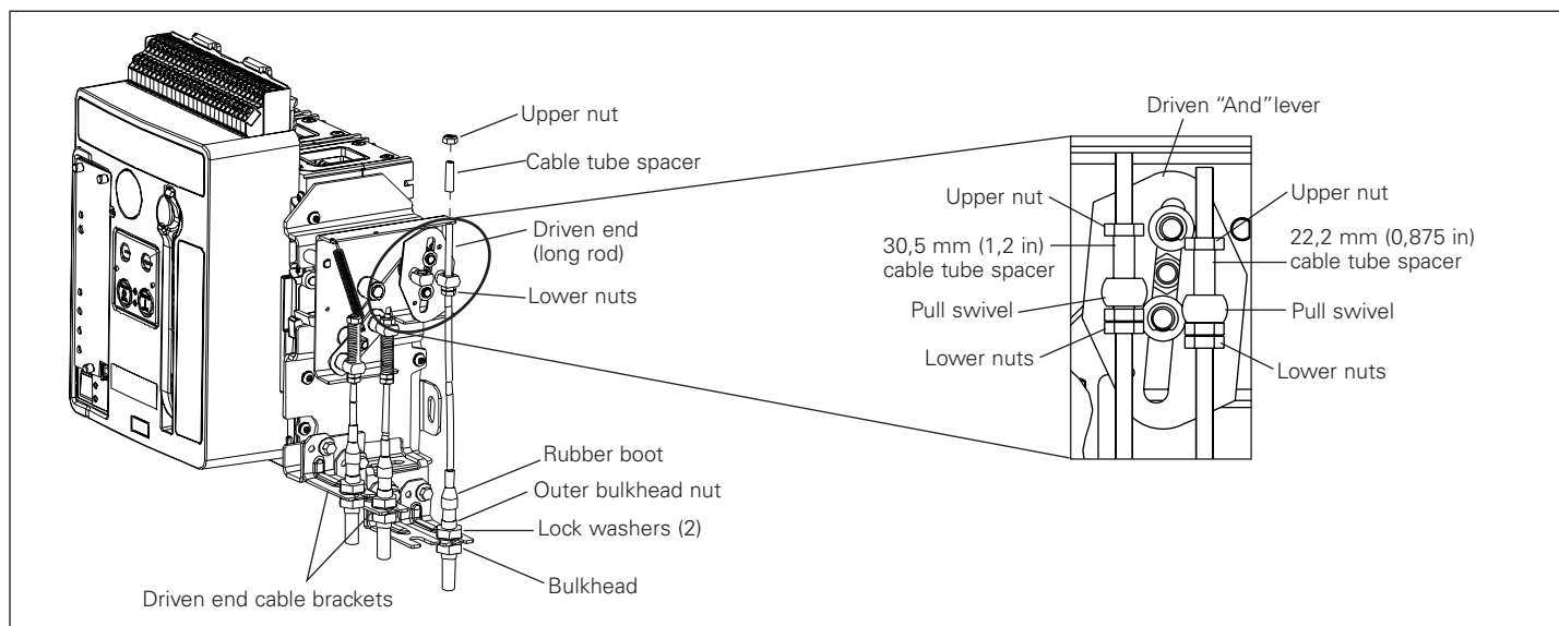
Figure 18. Details for Step 11: driven (long rod) end mounting component identification and Step 12 driven (long rod) end after adjustments
