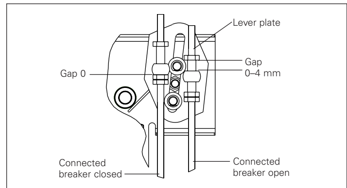
Figure 16. Driven "And" lever position with interconnected push breaker closed and pull breaker open
