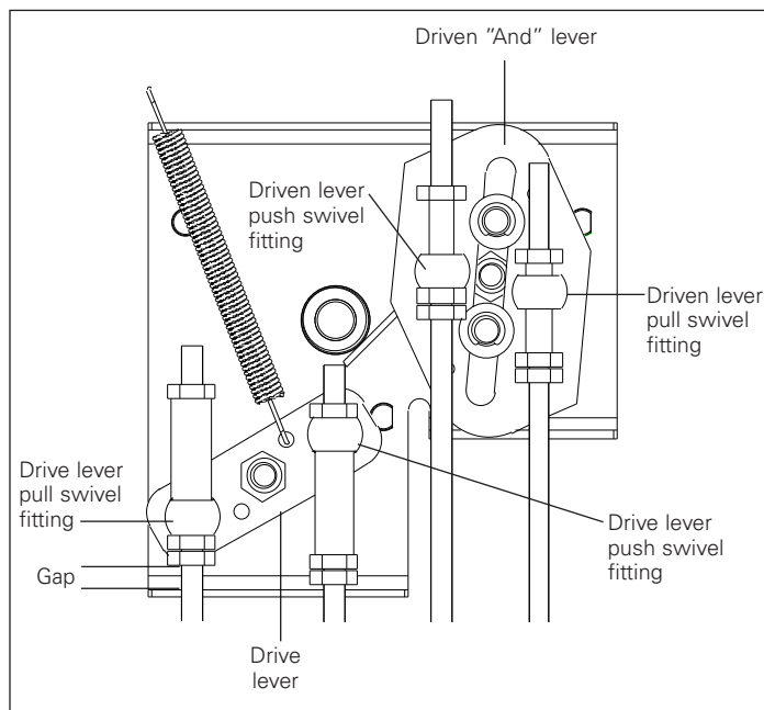
Figure 12. Push and pull swivel fitting identification
