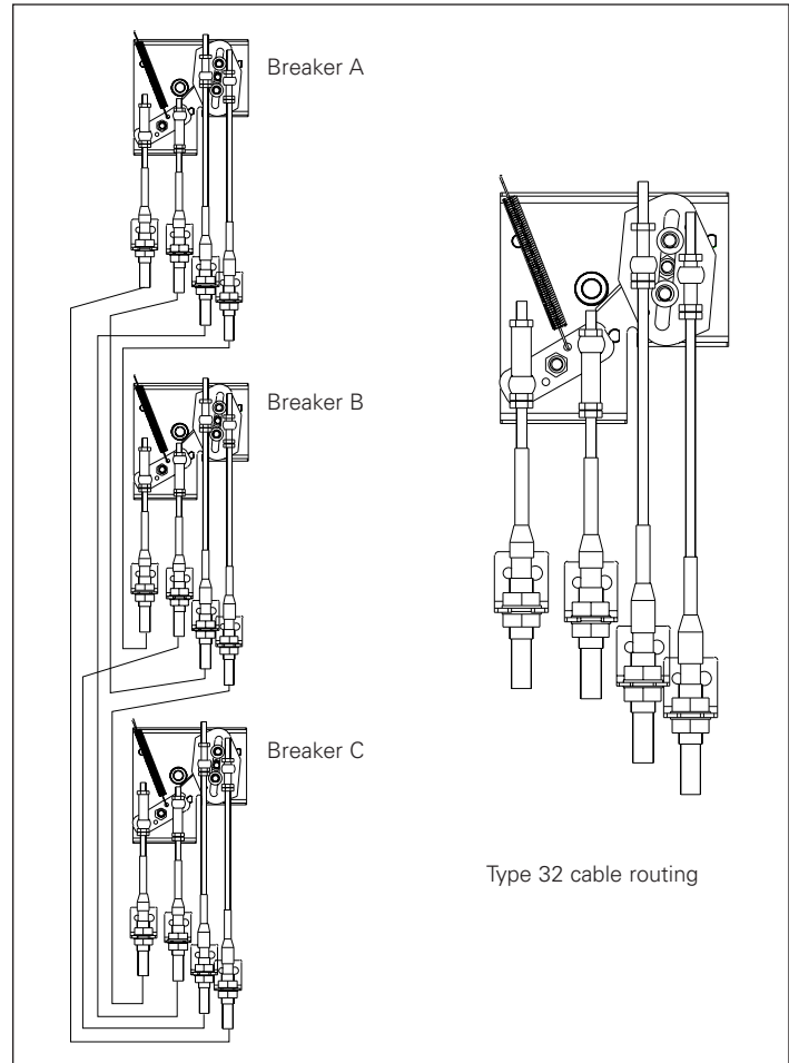
Figure 11. Cable routing for Type 32 interlock configurations
