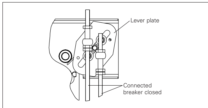
Figure 17. Driven "And" lever position with interconnected breakers closed
