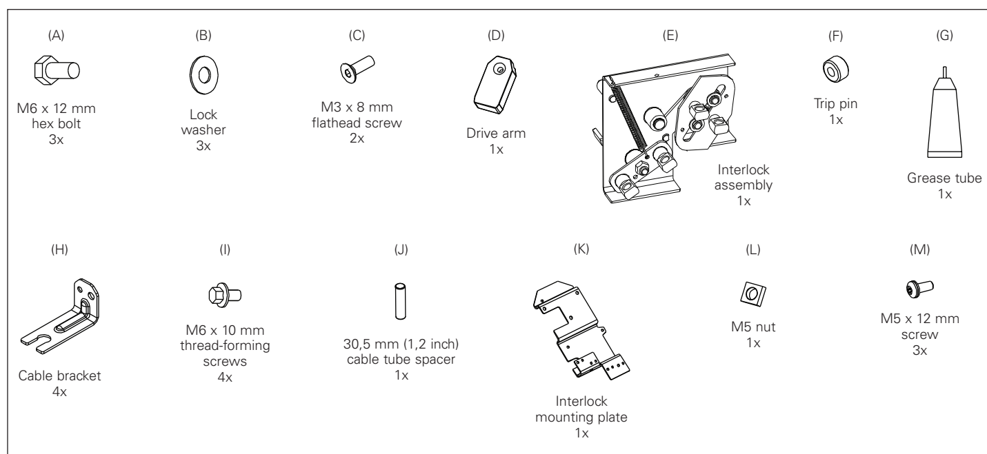
Figure 2. Interlock kit part identification, includes parts to install on a single fixed Type NF frame breaker and cassette (does not include cables)
