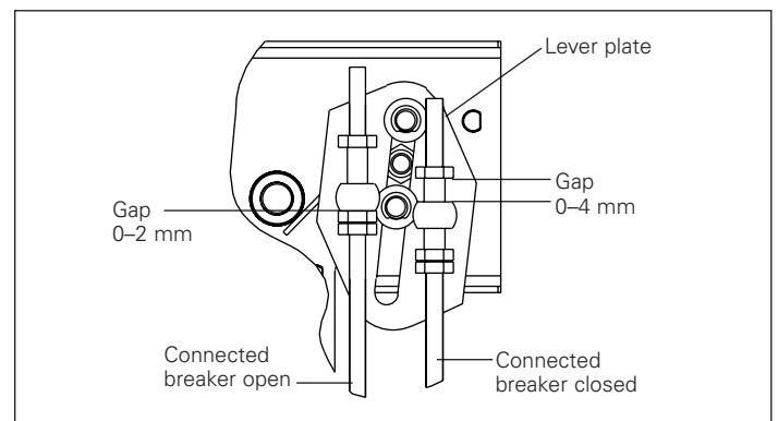
Figure 15. Driven "And" lever position with interconnected push breaker open and pull breaker closed
