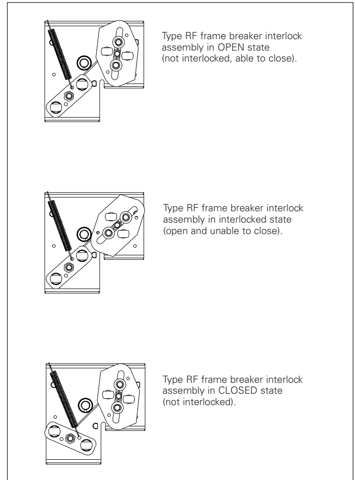
Figure 19. Position of interlock based on breaker state
