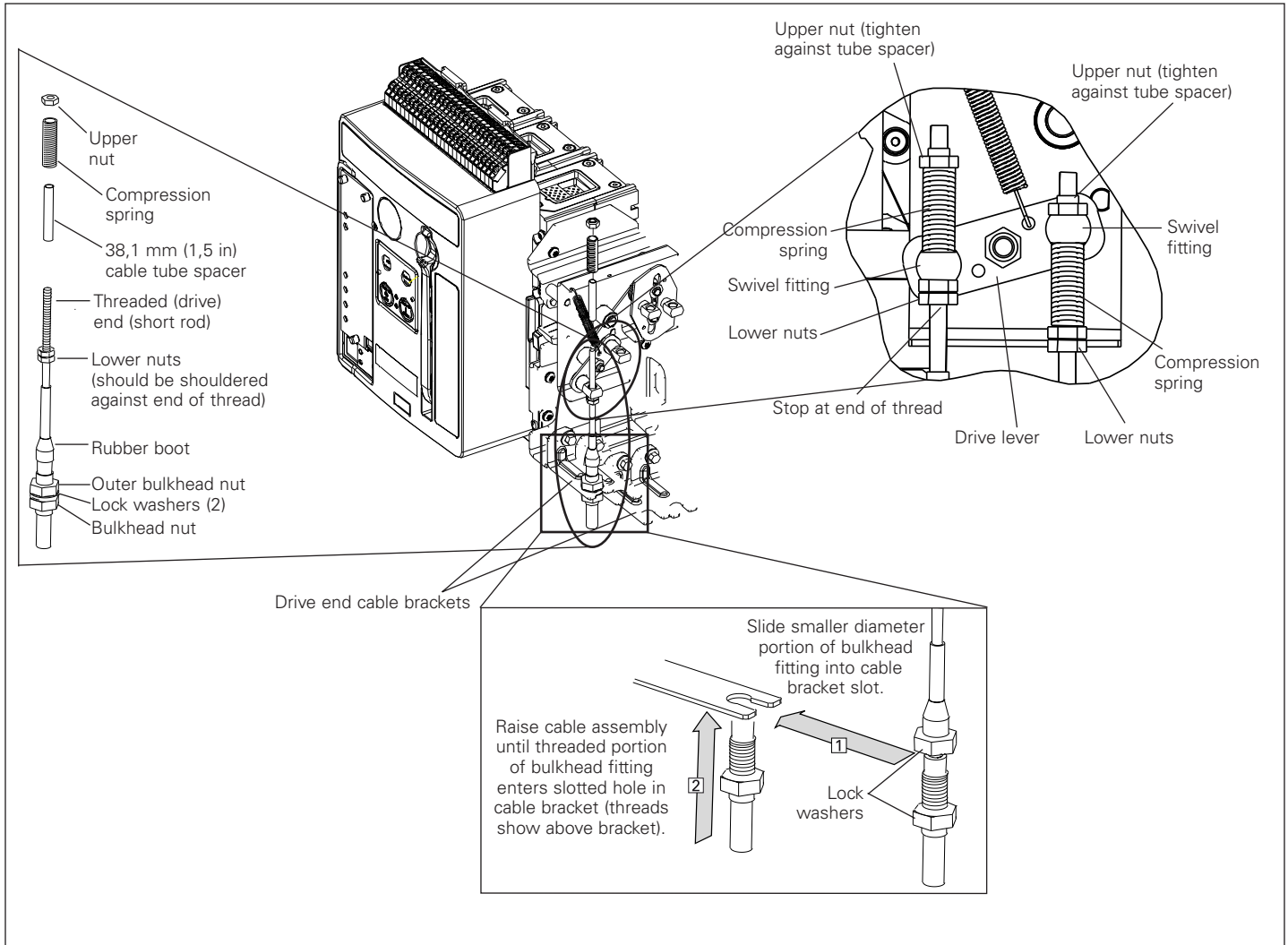
Figure 13. Details for Step 10: cable assembly drive (short rod) end mounting component identification, mounting cable assembly in cable bracket, and cable rod attachment to drive arm
