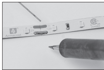
Splice Connection
