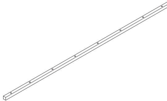
8 List x2 (1390x20x21mm) No. 12-02113901
