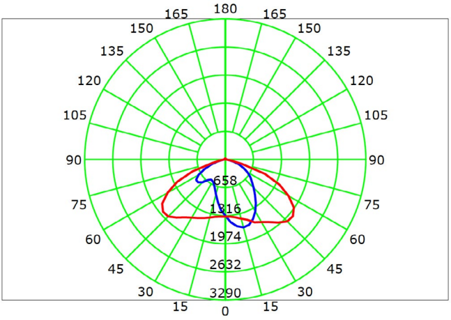
CEGONIA 30W Type III
