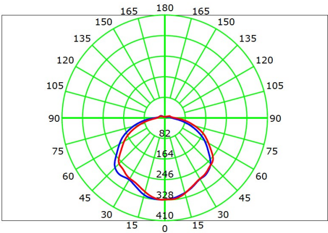
CEGONIA 20W Type III
