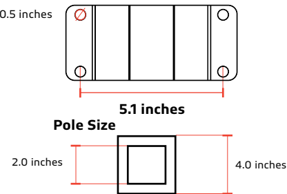
C-a. TLSTC-TRS-8W (for CEGONIA 8W) works with 2.0 inches to 4.0 inches poles.
