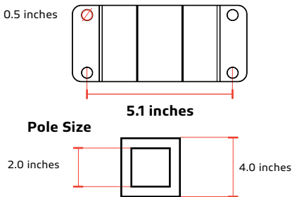
C-b. TLSTC-TRS-20W/30W (for CEGONIA 20W/30W) works with 2.0 inches to 4.0 inches poles.
