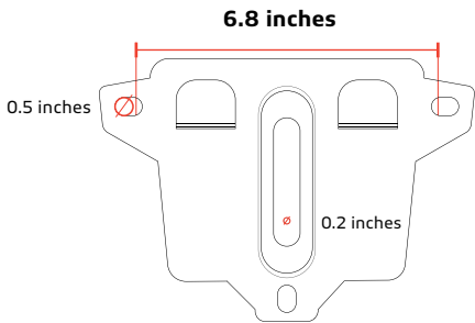
A-b. TLSTE-WM-20/30 (for CEGONIA 20W/30W)
