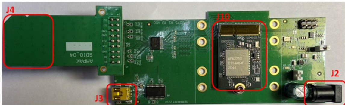
Figure1. Top view of WNFB-266AXI(BT) & AP12275_M2 EVB
