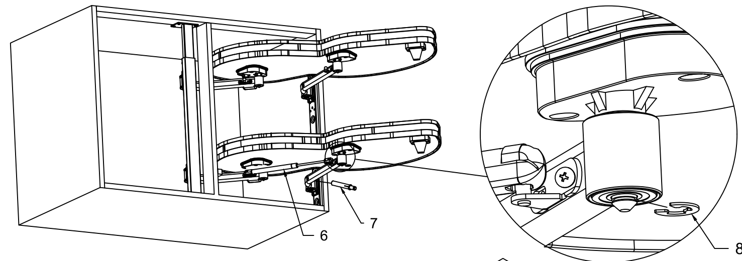
Drawing NO.2
