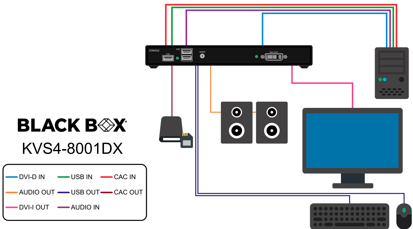
Figure 1-3: KVS4-8001DX
