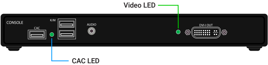
Figure 1-1: KVS4-8001DX Front panel
