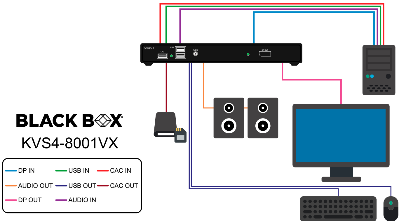
Figure 1-5: KVS4-8001VX
