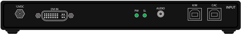
Figure 1-2: KVS4-8001DX Rear panel
