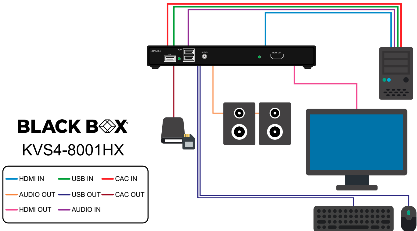
Figure 1-4: KVS4-8001HX
