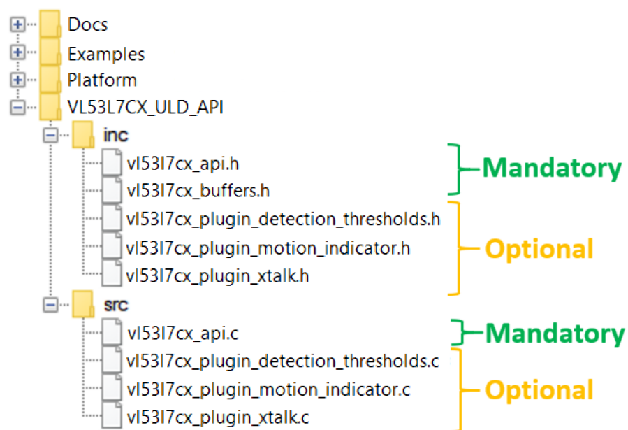
Figure 5. Driver architecture
