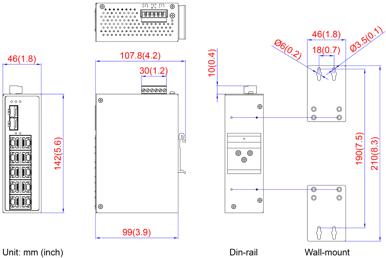
Figure 2.1: Physical Dimensions
