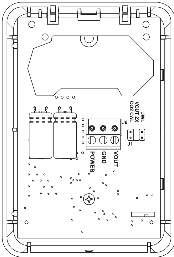
Fig. 5: Circuit Board
