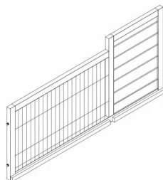
Back Panel- Left Side 1PC
