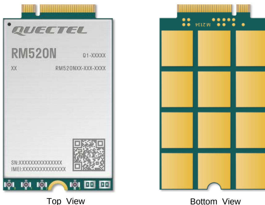
Figure 36: RM520N-GL Top and Bottom Views
