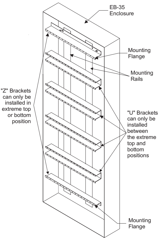
Figure 1 Installing the EK- Rail Kits
