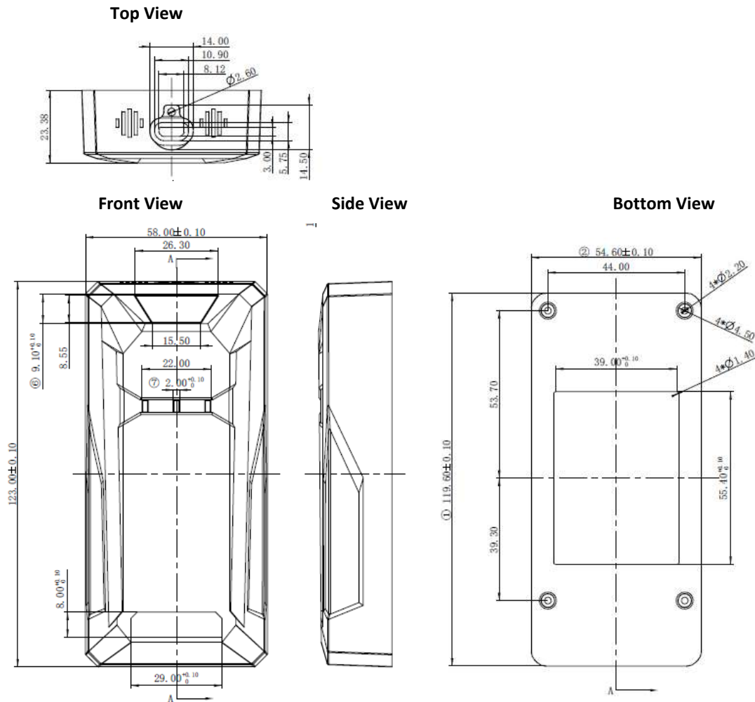
Figure 4-1 Mechanical Drawing
