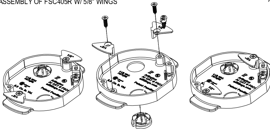
ASSEMBLY OF FSC405R W/ 5/8" WINGS
