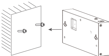
Figure 2-1 Wall-Mounted Installation
